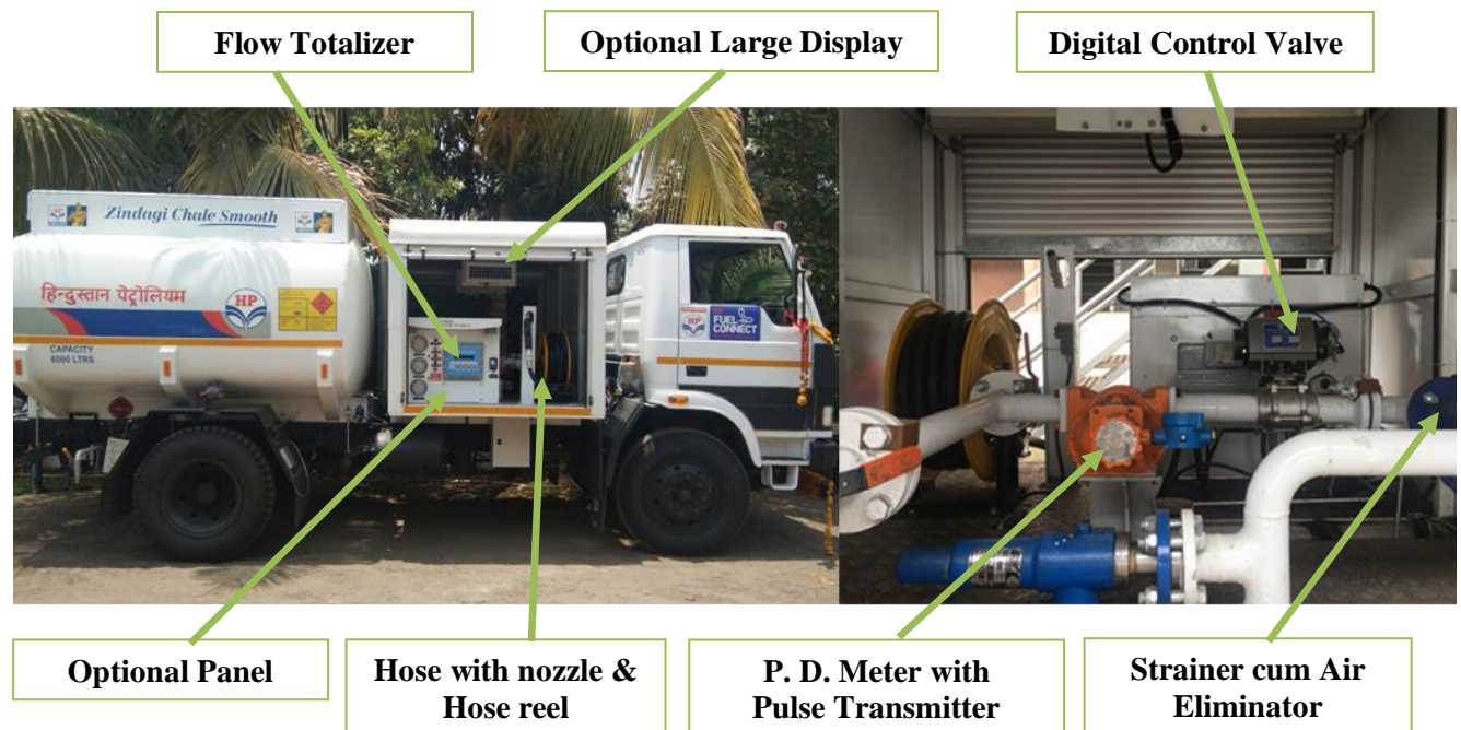
P. D. Flowmeter in Bowser Truck dispensing application
